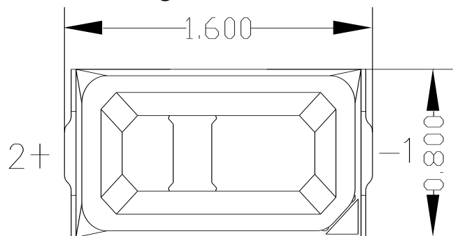
Fig.1-1 Top view
