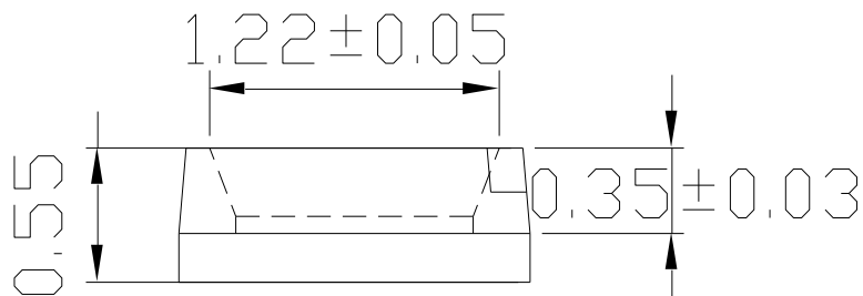
Fig.1-2 Side view
