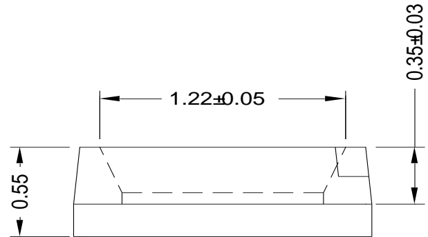
Fig.1-2 Side view
