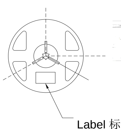
Fig.2-2 Reel Dimension 卷盘尺寸
