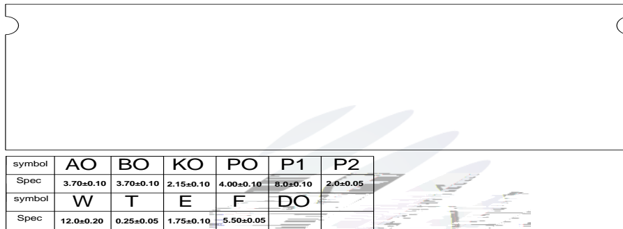
Fig.2-1 Carrier Tape Dimension 载带尺寸
