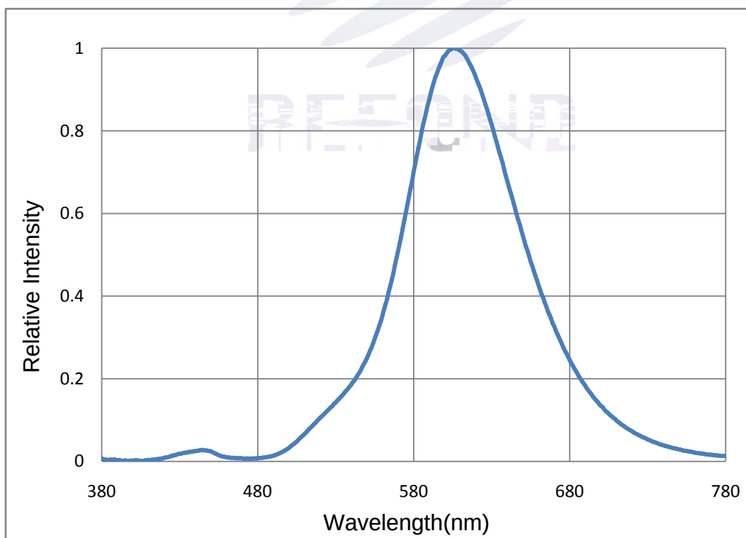
Fig. 1-14 Spectrum Distribution
