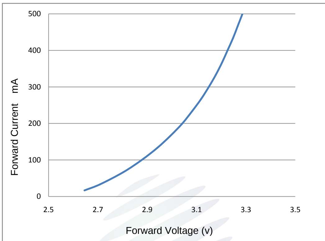
Fig. 1-7 Forward Voltage Vs Forward Current
