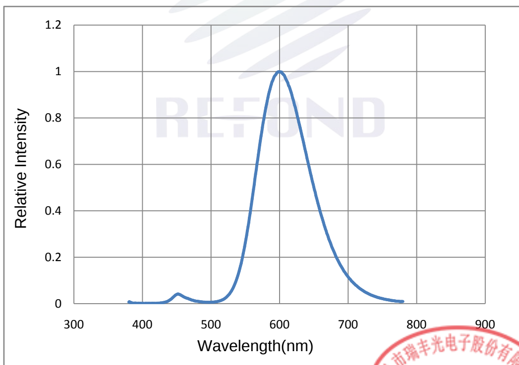
Fig. 1-14 Spectrum Distribution
