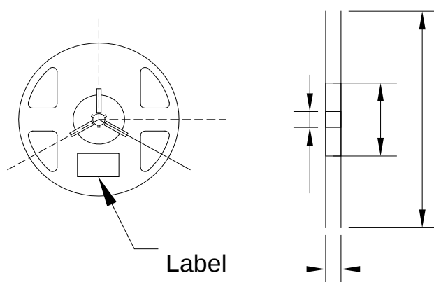
Fig.2-2 Reel Dimension
