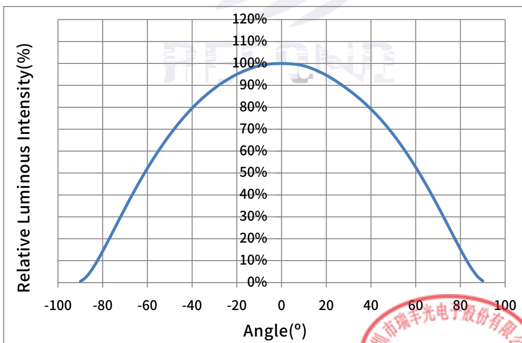
Fig. 1-12 Radiation diagram
