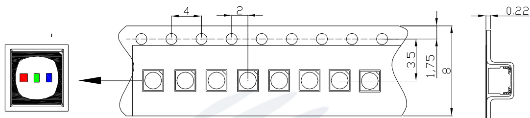
Fig.2-1 Carrier Tape Dimension
