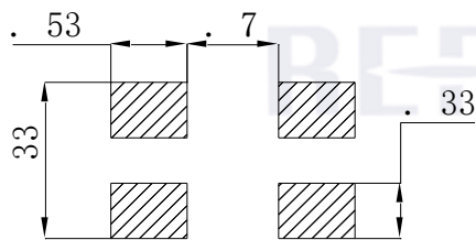
Fig.1-5 Soldering patterns
