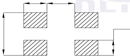
Fig.1-5 Soldering patterns
