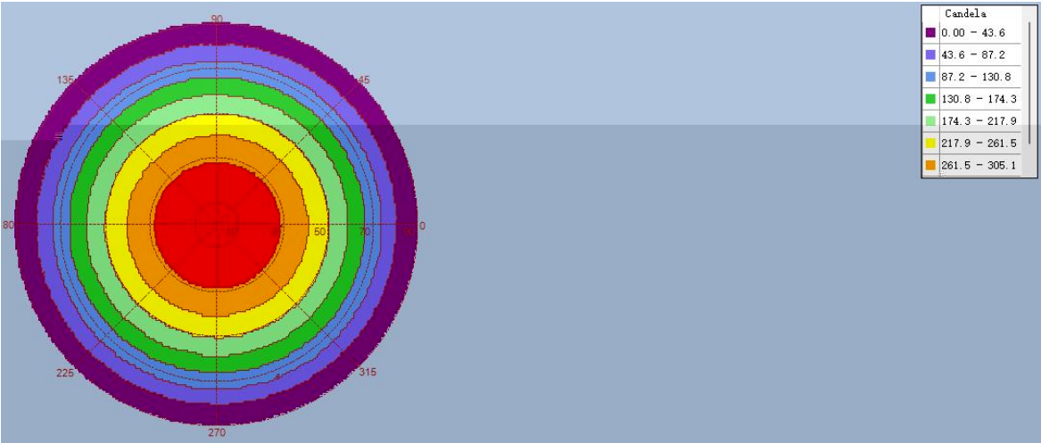
Intensity(traced to infinity) Iso-Plot
