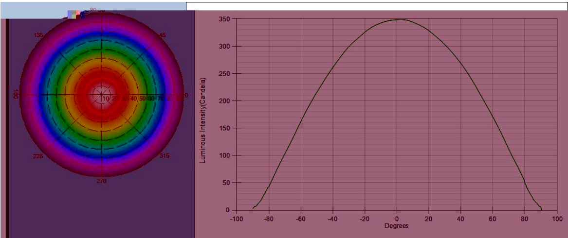
Intensity(traced to infinity) Cross Section Luminous Intensity(Candela)
